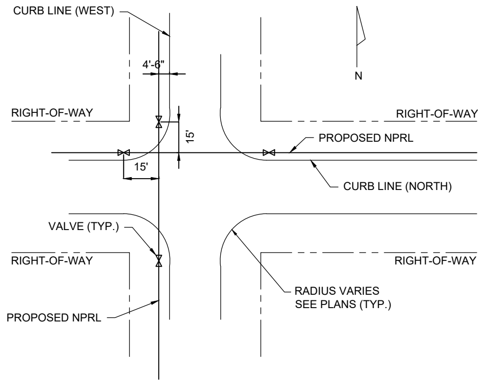
SUBDIVISION INTERSECTION DETAIL VALVE & MAIN NTS
