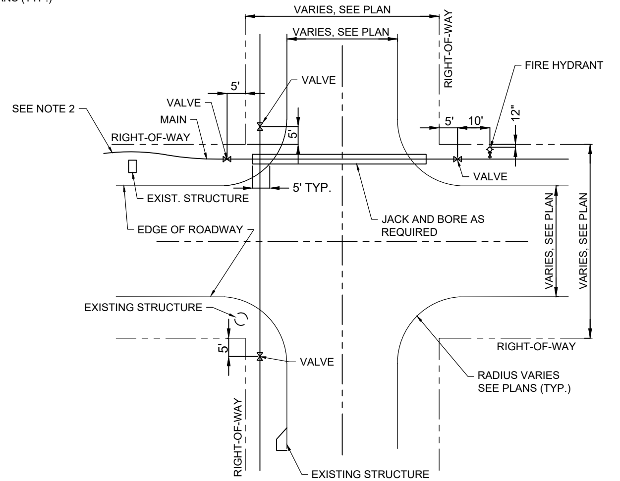
TYPICAL WATER MAIN AT INTERSECTION NTS
