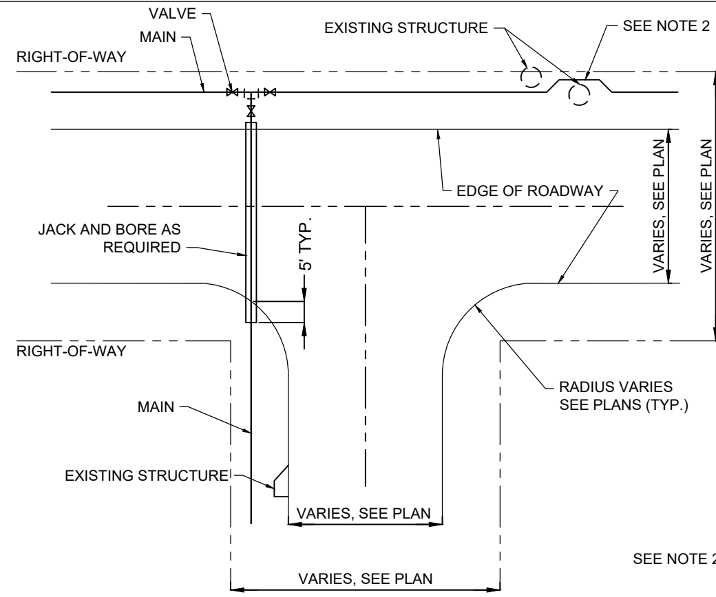
TYPICAL BRANCH CONNECTION AT INTERSECTION NTS
